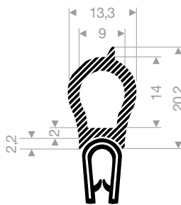
pvc + sponge rubber clamping range 9-10,5 mm roll length 50 meter
